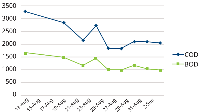
Figure 1- COD & BOD in mg/l at ETP Outlet
